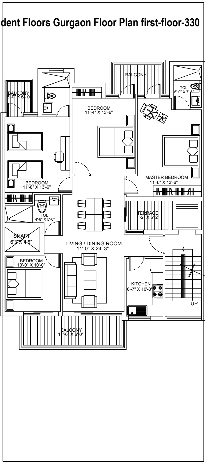
FIRST FLOOR
